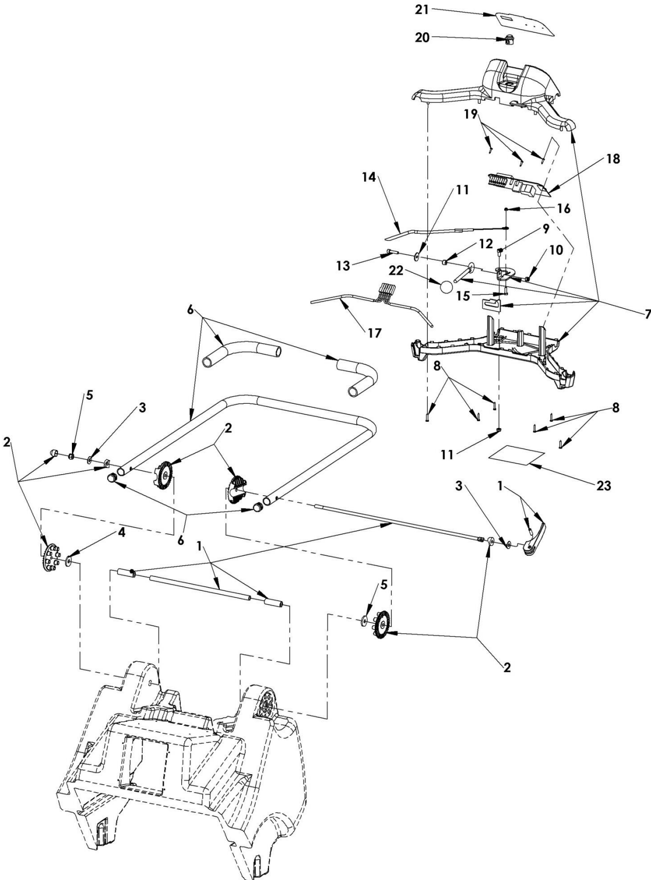
Fig. 4 – Handle Assy
