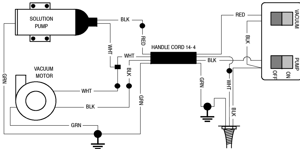
WIRING DIAGRAM, 220V/230V
