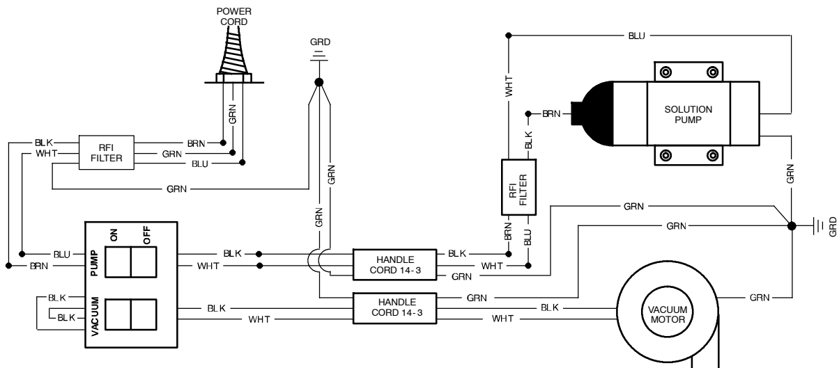
WIRING DIAGRAM, 240V EMC MODEL
