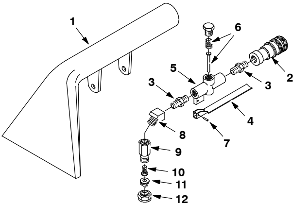
HAND TOOL, 127 mm (5 in)
